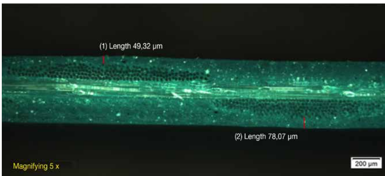
Competitor X: (1) front face 50 μm (2) rear face 78 μm
