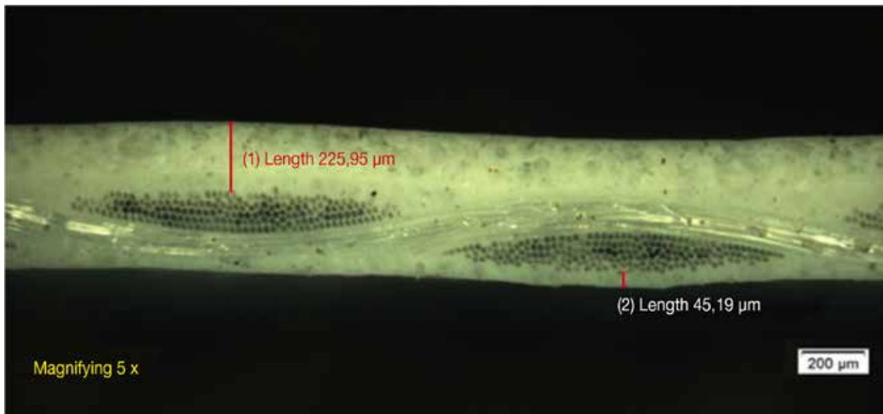
Serge Ferrari: Protect Cover 505 (1) front face 225 μm (2) rear face 45 μm
